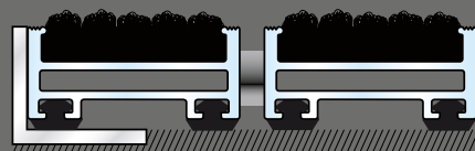
Top Clean STABIL XL 22 and 27 mm
