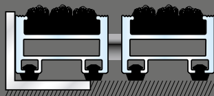
Top Clean STABIL 10, 17 and 22 mm
