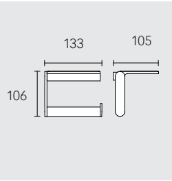
Toilet paper holder
