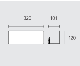
Shower shelf wall mounted, removable, with concealed fastening, integrated drain slots and hooks 24952 370000
