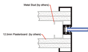
SG Wraparound Conversion
