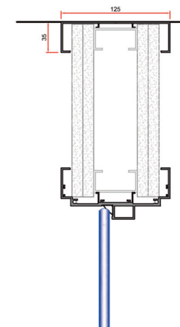
Drywall Doorframe Head - Glass
