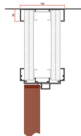
Drywall Doorframe Head - Timber
