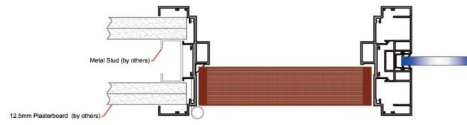
Drywall Conversion - Timber
