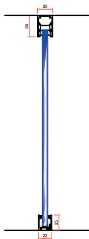
SG 35mm Head & Base
