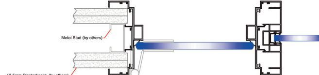
Drywall Conversion - Glass
