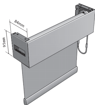
75mm Square Facia
