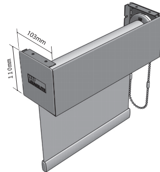
100mm Square Facia
