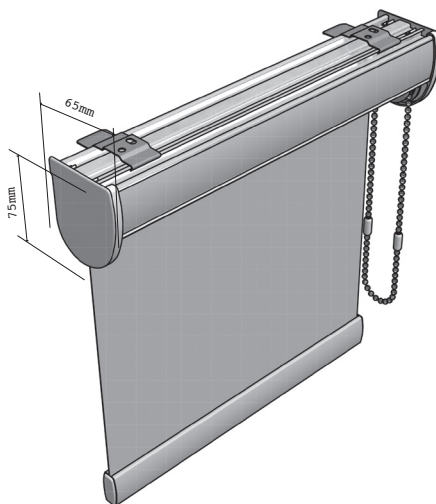
Open Cassette system
