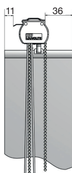
TOP FIX BRACKETS (SPRING)
