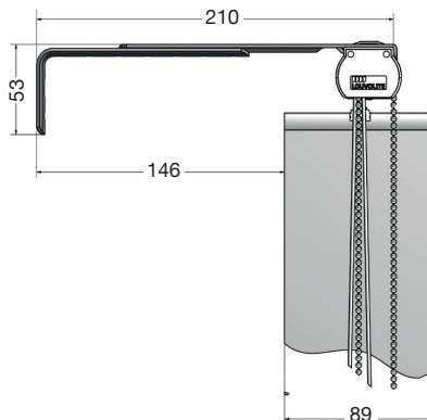
ADJUSTABLE FACE FIX BRACKETS
