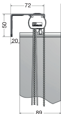
SHALLOW FRAME FACE FIX BRACKETS
