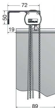
SHALLOW FRAME FACE FIX BRACKETS
