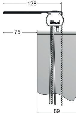
EXTENSION TOP FIX BRACKETS
