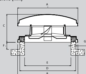
Dimensions (mm)
