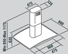
90 Island
