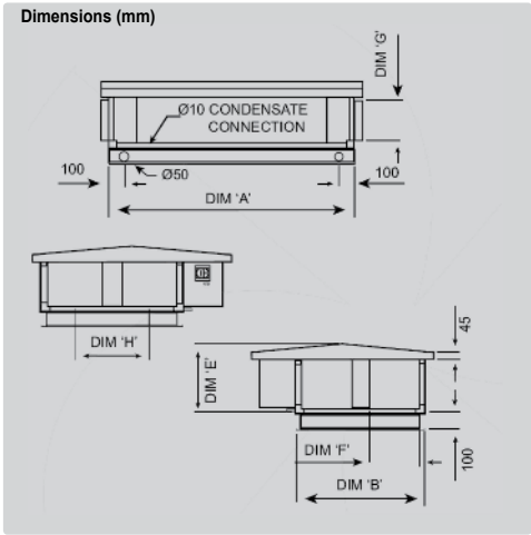
Dimensions (mm)
