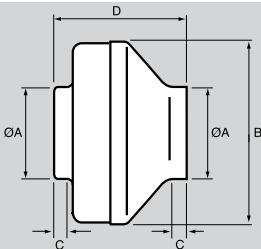
Dimensions (mm)
