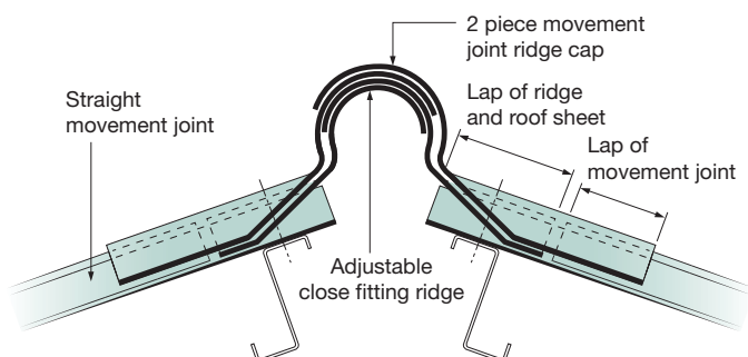
Fig.3 - Movement joint ridge cap
