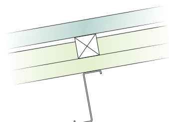
Fig.5 - Rigid insulation board, timber spacer and second insulation layer
