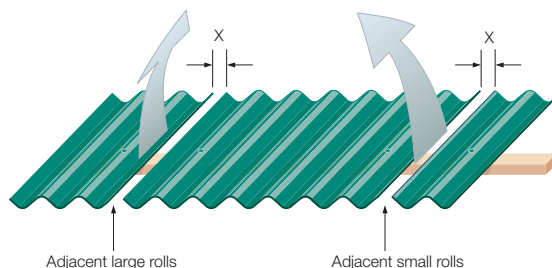
Fig.4 Spaced roof
