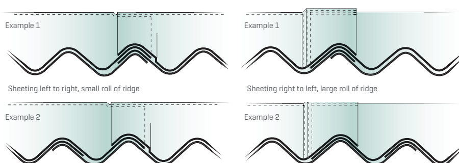
Fig.2 - Two piece plain wing ridge
