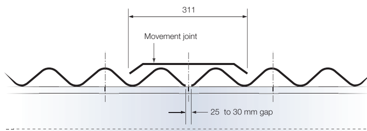
Fig.4 - Vertical movement joint
