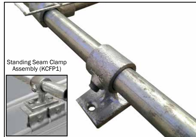
K. Slide 1No. Rail Support fitting over each end of the exposed tube in the corners of the frame. Carefully align the fitting to ensure it is positioned on the crown of roof sheet. NB If attaching to standing seam roof use KCFP1 clamps to connect to the standing seam and bolt the 70-5 fitting to the KCFP1 clamp as shown in the diagram and proceed to step L .
