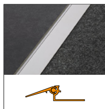
Schlüter®-RENO-V
