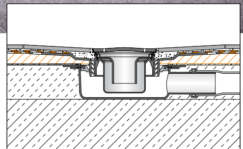
Horizontal drainage
