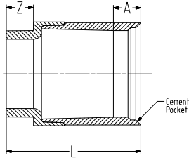
Socket Coupling and Closure Coupling
