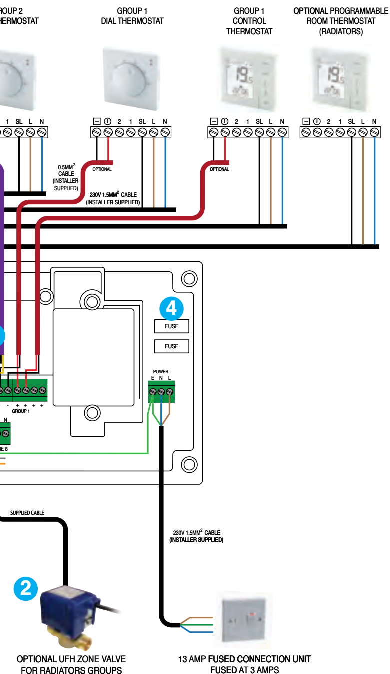
230v Dial Thermostat Part No. JGSTAT1
