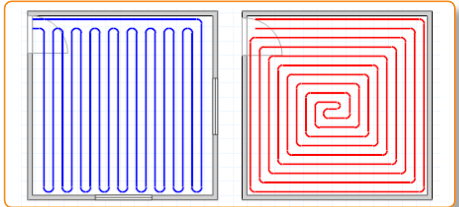
Diagram 1 - Serpentine is a simple up & down circuit pattern. It is especially good to use when you have irregular shaped rooms or small areas such as kitchens and utility rooms.
