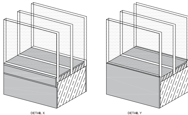
DETAIL X
