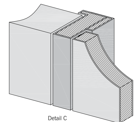
Detail C
