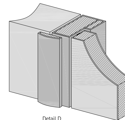
Detail D
