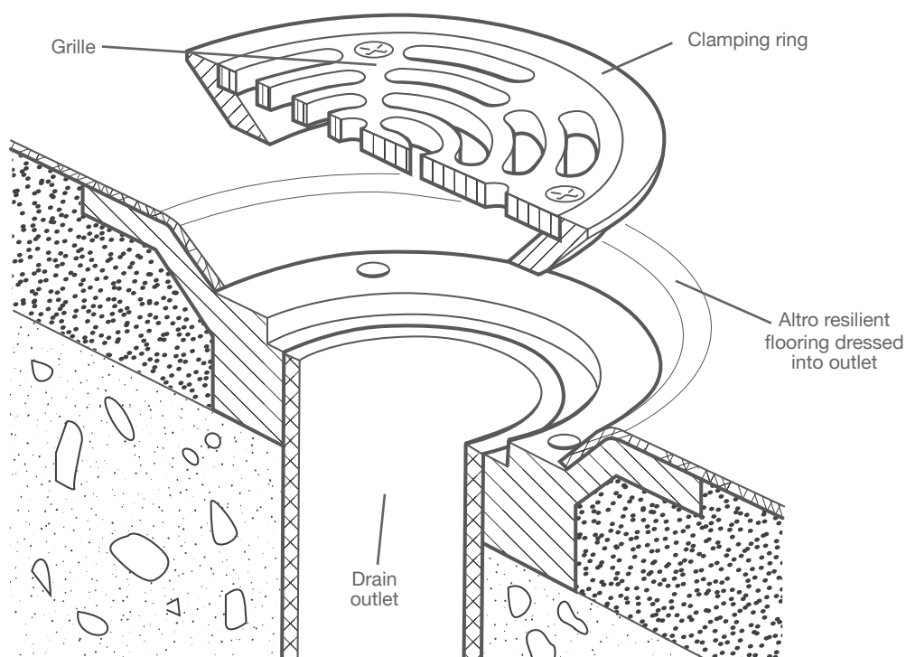
Transition with clamping channel
