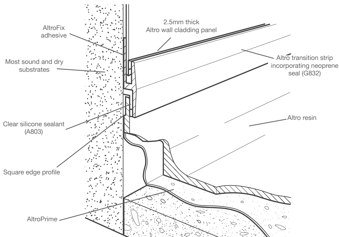
Altro wall system to Altro resin flooring detail
