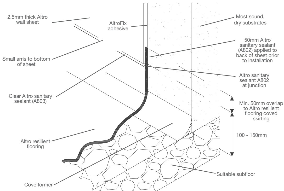
Altro wall system to Altro resilient flooring overlap detail
