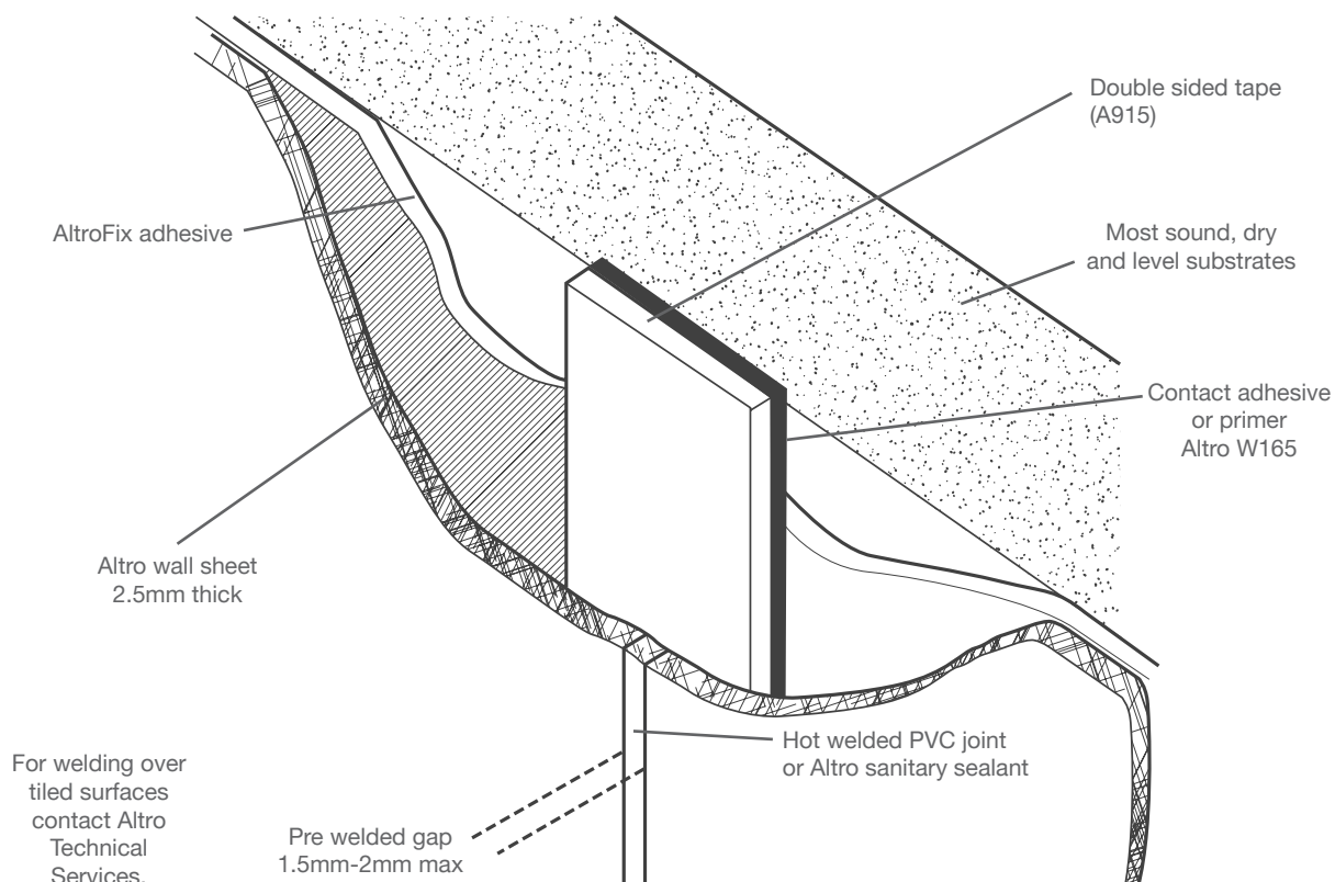
Altro wall sheet to Altro Whiterock FlexiJoint detail
