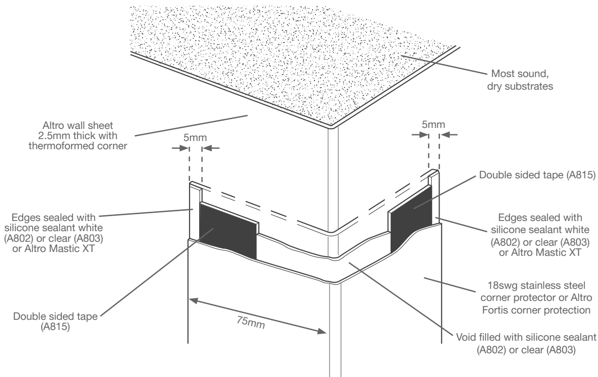
Altro wall system with corner protector fixing detail
