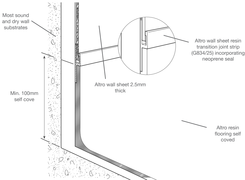
Altro wall system to Altro resin flooring detail
