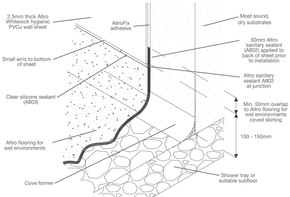
Altro Whiterock hygienic PVCu wall system to Altro flooring for wet environments shower tray detail
