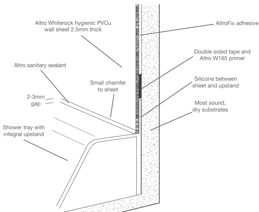
Altro Whiterock hygienic PVCu wall system to shower tray with integral upstand detail
