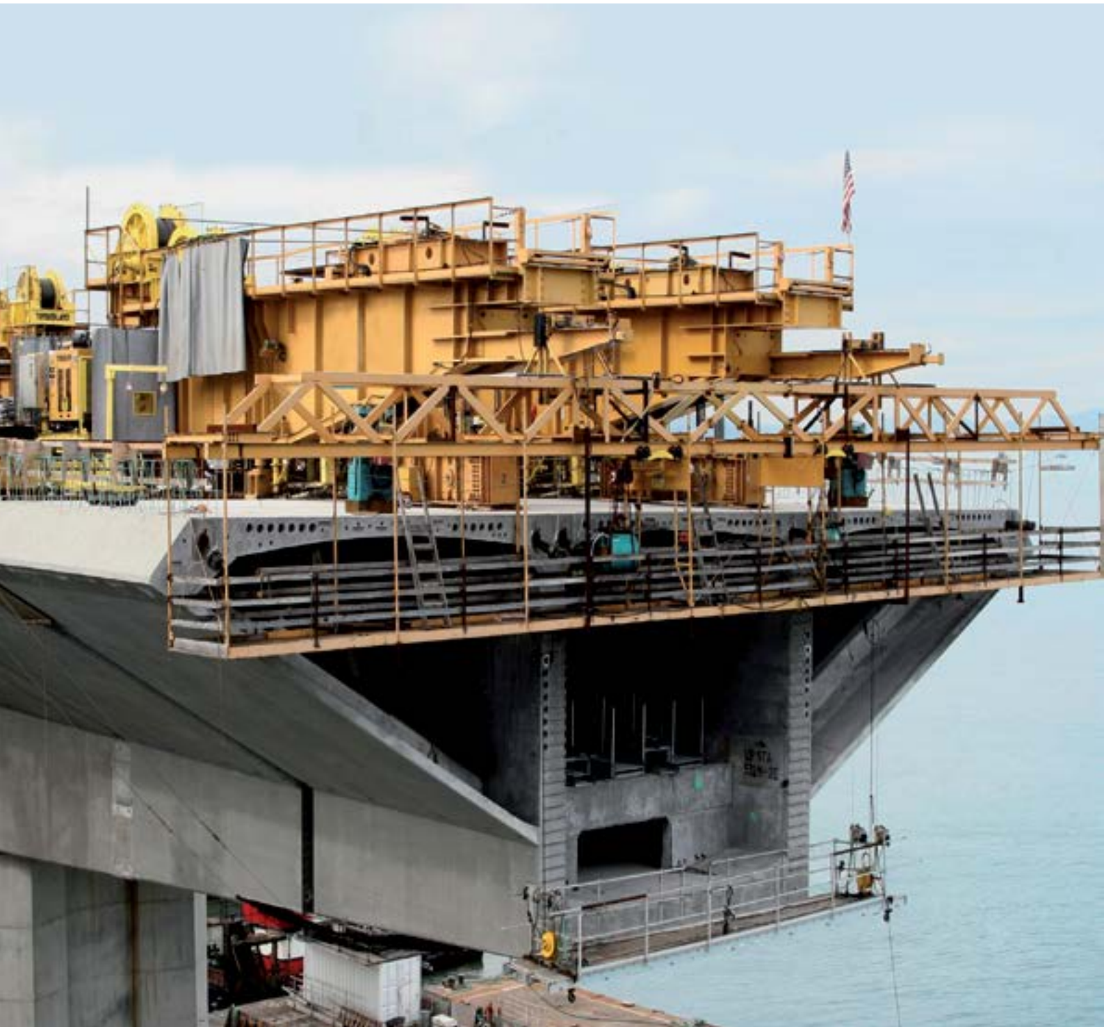
Structural bonding solution for a segmental bridge, Oakland Bay Bridge, San Francisco, USA
